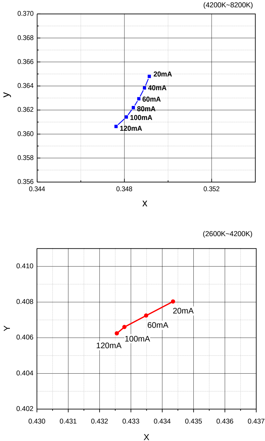
Fig 5. Forward Current vs. CIE X, Y Shift , T_a = 25^\circ\text{C}
