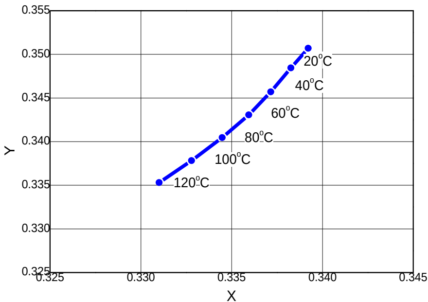
Fig 8. Chromaticity Coordinate vs. Junction Temperature I_F=100\text{mA} (4200K~8200K)
