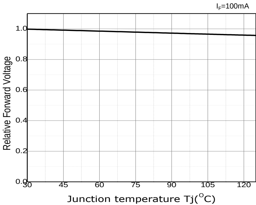
Fig 7. Junction Temperature vs. Relative Forward Voltage
