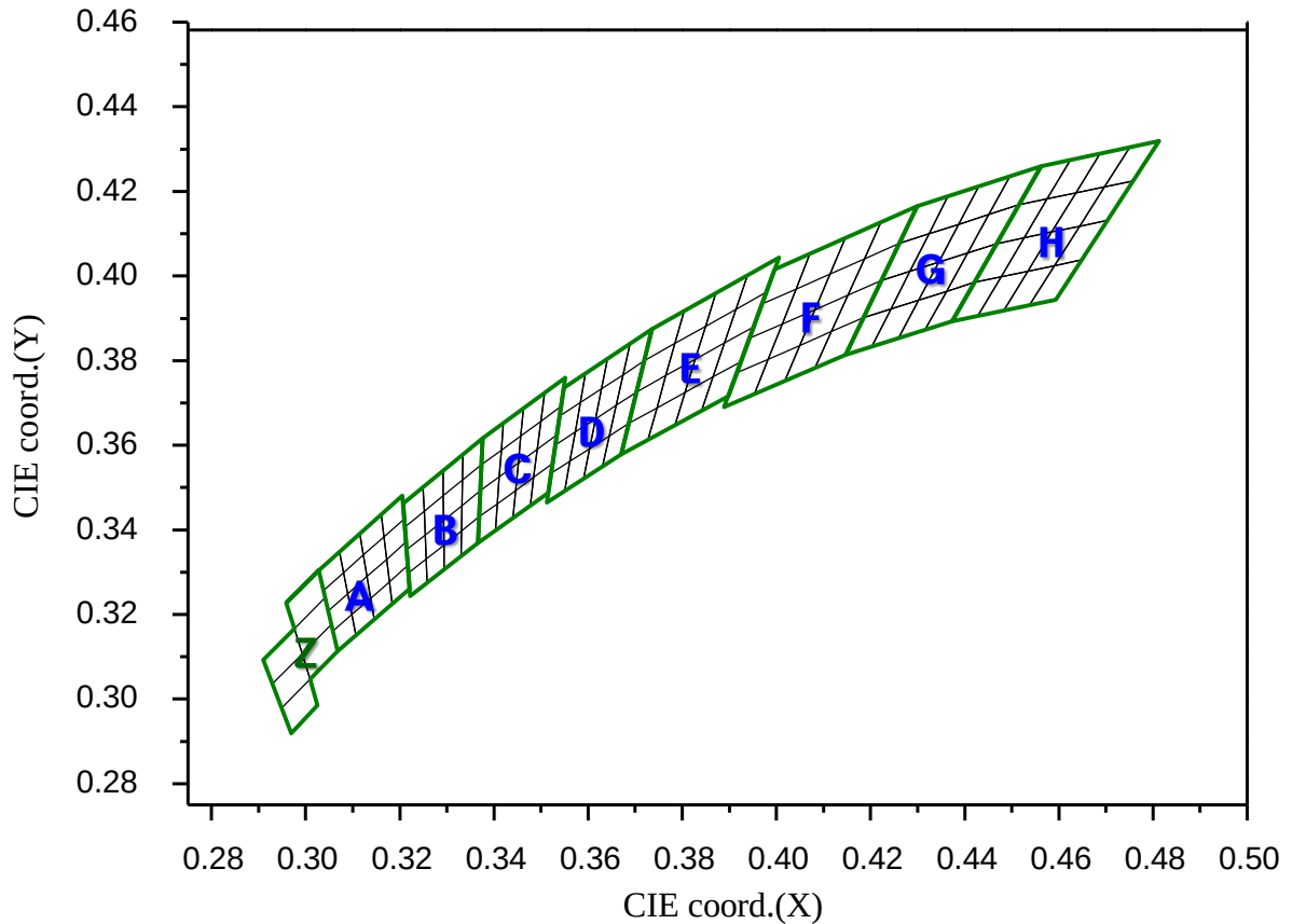
Fig 10. CIE Chromaticity Diagram T_a=25^{\circ}\text{C} , I_F=100\text{mA}
